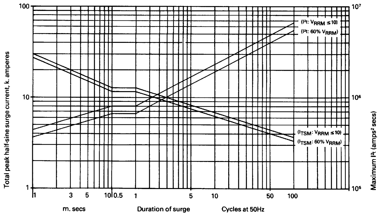
Figure 6 Max. non-repetitive surge current at initial junction temperature 125°C.
