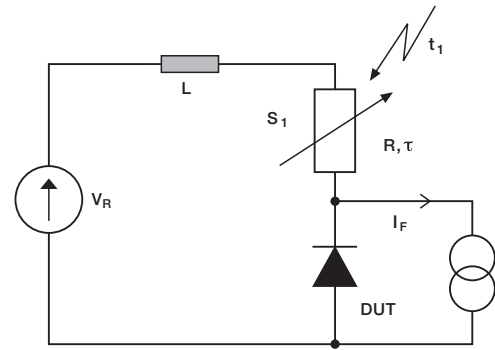
Fig. 2b Resistive commutation
